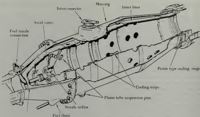
FIGURE 1-44. Can-type combustion chamber.
